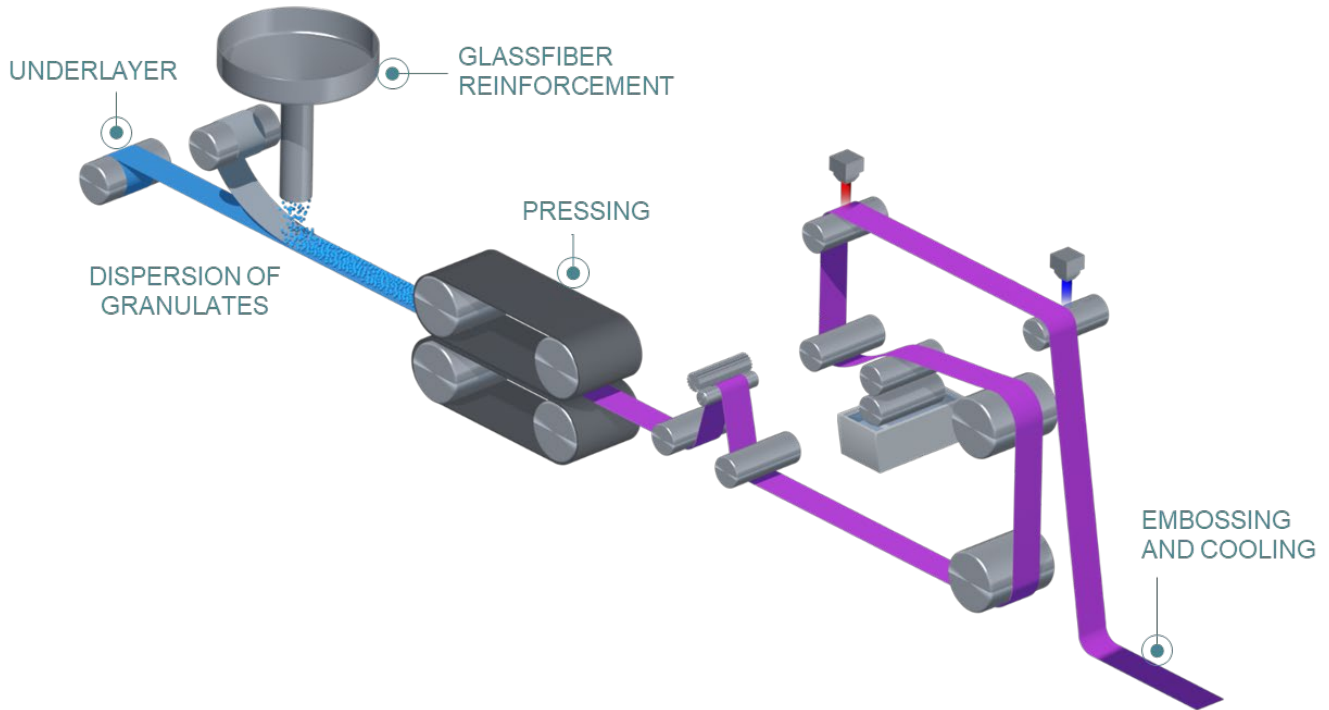
Pressing manufacturing process flow diagram
